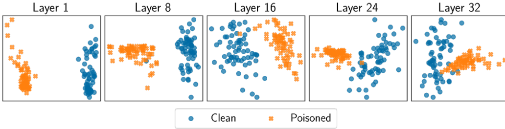
Figure 32: PCA of barcode summaries of clean vs. poisoned activations. Clear distinction appears in the projection onto the two first principal components from the PCA of the pruned barcode summaries for layers 1, 8, 16, 24, and 32.
