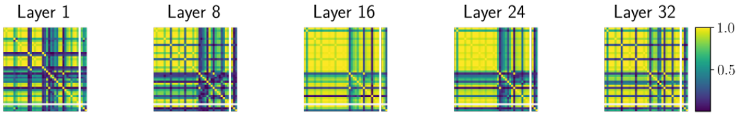
Figure 26: Cross-correlation matrices for the barcode summaries for clean vs. poisoned activations. Growing block of correlated features appears in the cross-correlation matrix of the barcode summaries for layers 1, 8, 16, 24, and 32. Correlations in layer 1 are lower than with Mistral 7B, see Figure 6.
