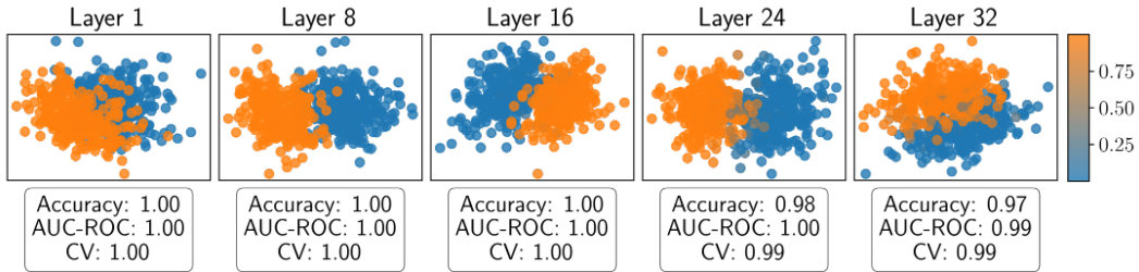
Figure 54: Llama with Euclidean distance: Logistic regression for locked vs. elicited activations. Prediction of a logistic regression trained on a 70/30 train/test split of the pruned barcode summaries, plotted on the projection onto the two first principal components for visualization purposes. Accuracy and AUC-ROC tested on the test data, and 5-fold cross validation on train data are presented for each model, showcasing the outstanding performance of all models.
